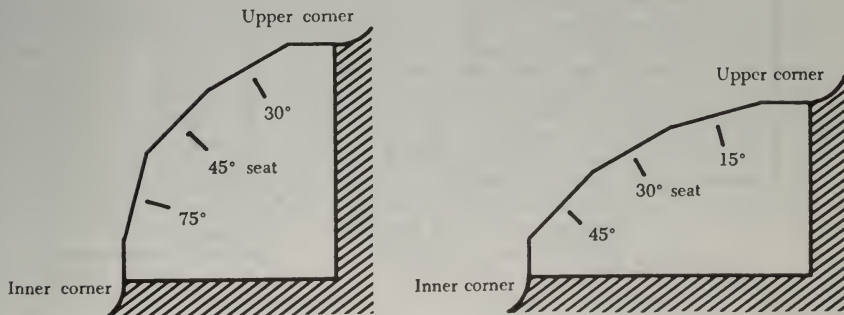
FIGURE 10-13. Valve seat angles.
